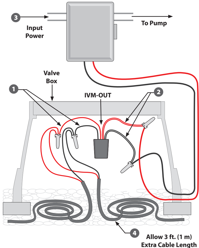
Typical IVM-OUT Pump Start Relay Wiring
