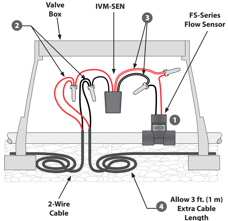
Typical IVM-SEN Flow Sensor Wiring
