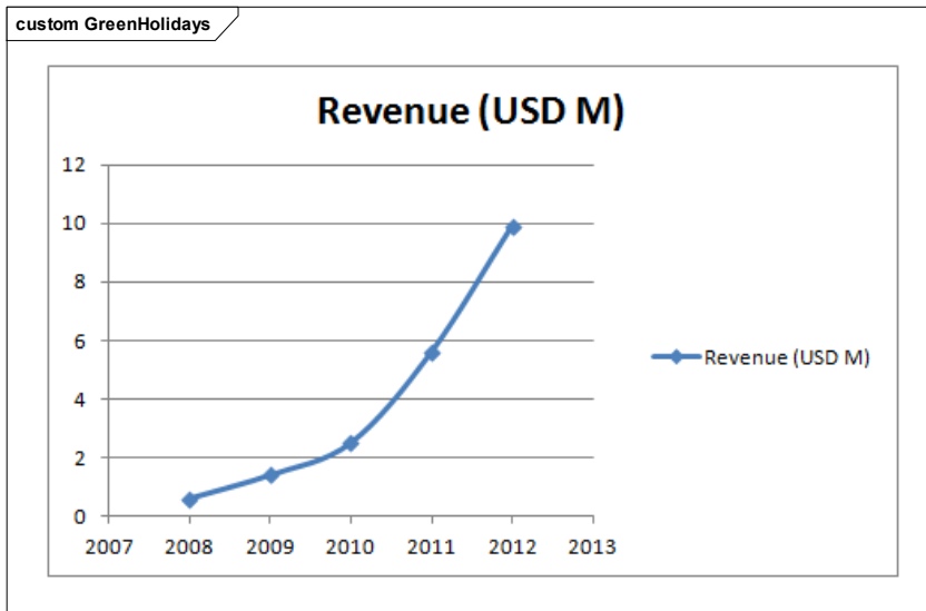
Figure 2 : GreenHolidays
