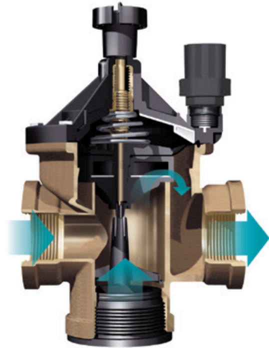
BPES Cutaway
