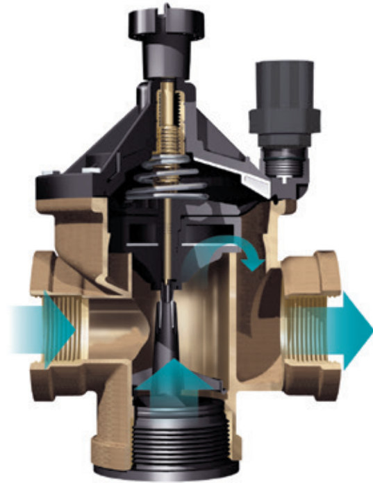
BPES Cutaway
