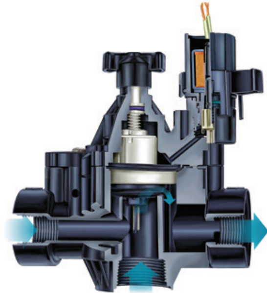
PGA Cutaway
