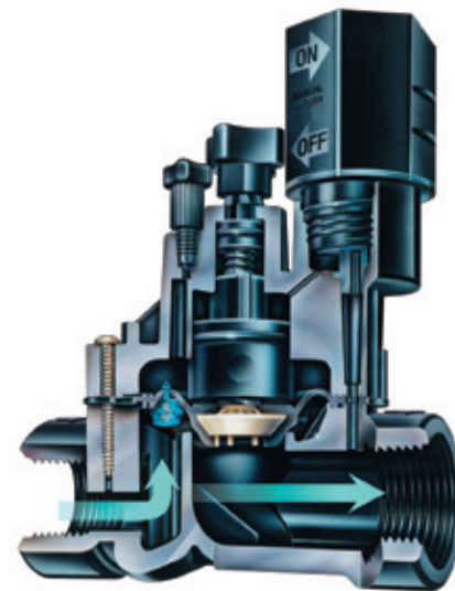
DVF Cutaway
