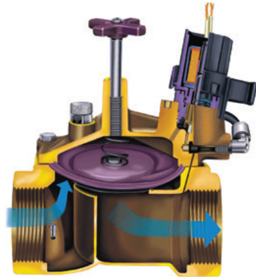
EFB-CP Cutaway
