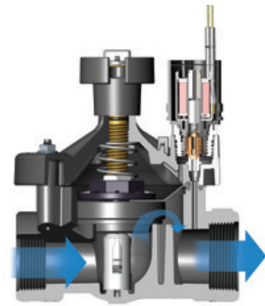
PESB Cutaway
