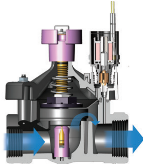
PESB-R Cutaway
