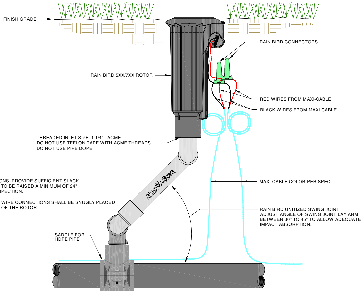
○ RAIN BIRD 5XX/7XX IC ROTOR ON TOP MOUNT SADDLE NOT TO SCALE
