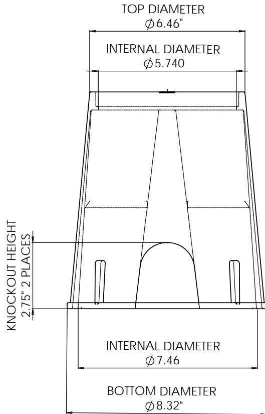
6" ROUND VALVE BOX DIMENSIONS
