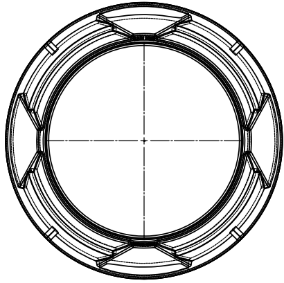
6" ROUND VALVE BOX DIMENSIONS
