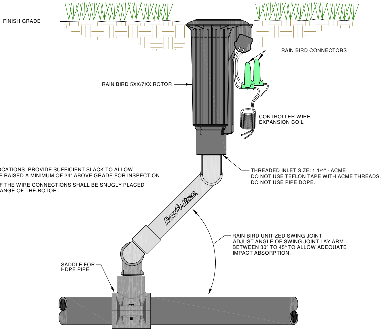
RAIN BIRD 5XX/7XX ROTOR ON TOP MOUNT SADDLE NOT TO SCALE
