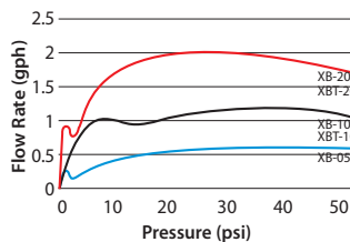
Xeri-Bug Emitter Performance
