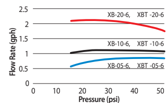
Multi-Outlet Xeri-Bug Emitter Performance
