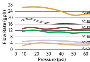
Pressure-Compensating Modules Performance
