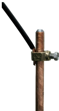
FIGURE 5-14. The #4 cable connected to the ground rod
