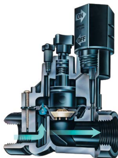
DVF Cutaway
