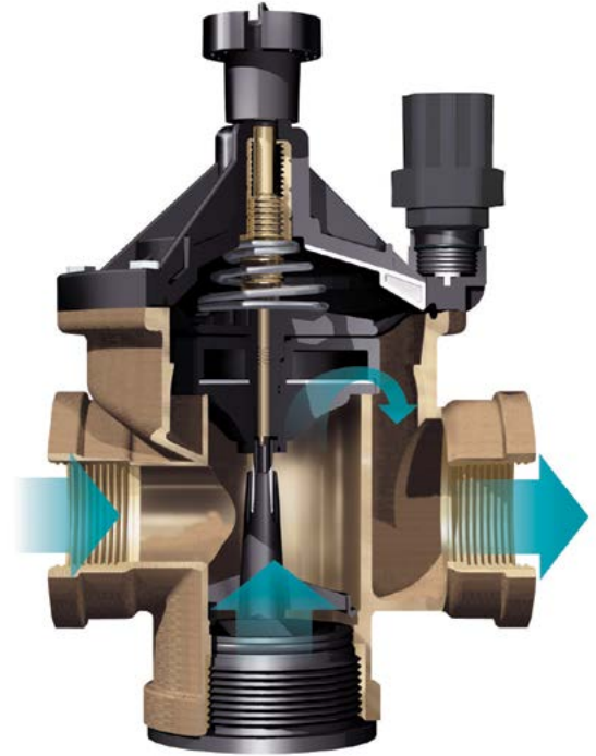
BPES Cutaway
