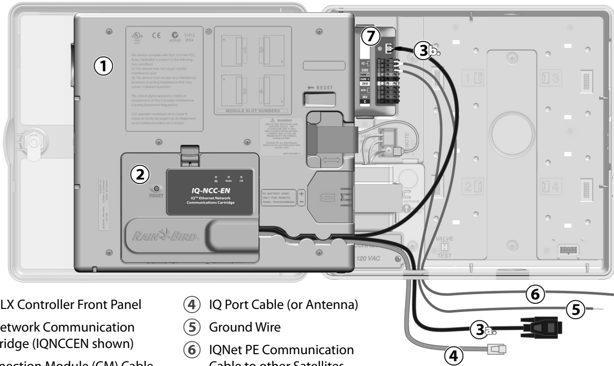
Figure 2 - Installation Overview
