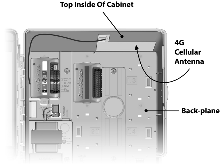
4G Cellular Internal Antenna Installation
