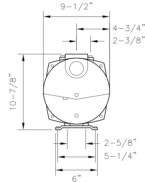
3-HP HEAVY DUTY PUMP
