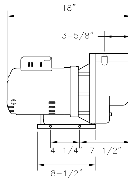
3-HP HEAVY DUTY PUMP
