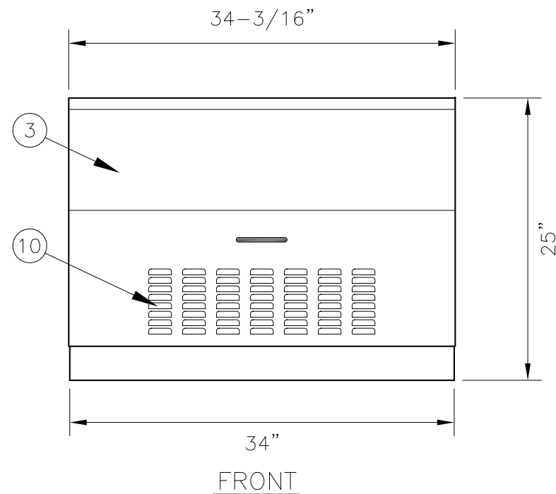
STEEL ENCLOSURE
